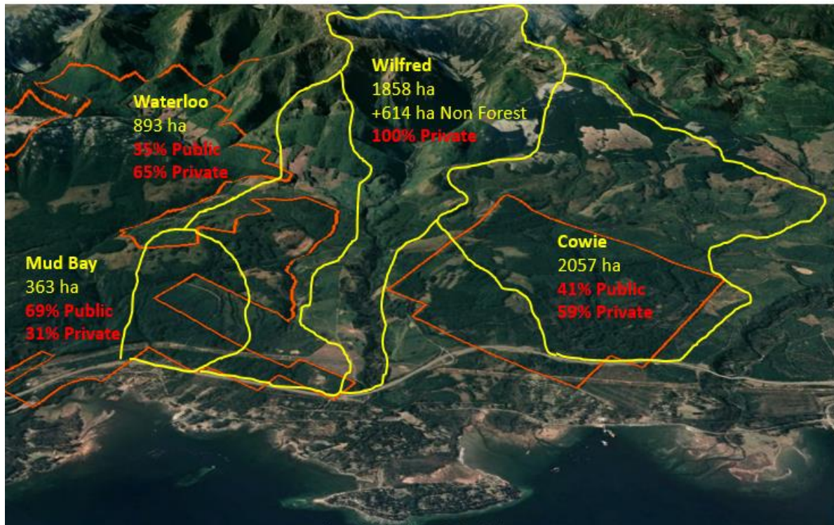
Figure 1: Oblique 2020 Google Earth image of the 4 studied watersheds (Watershed boundaries and areas are in yellow; public land boundary is in orange; percent public and private land are in red).
